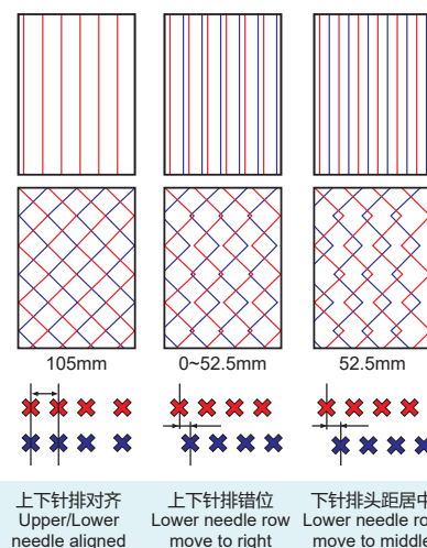
105mm头距双针排机型排针效果 105mm Head distance double row pattern
